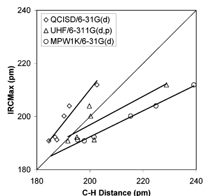
Figure 4. Bond lengths (pm) of the forming C–H bond in the transition state of the hydrogen radical addition to alkenes: values from various levels of theory versus IRCMax(CBS-QB3/B3LYP/6-311G(d,p)) values.
