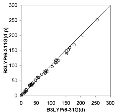
Figure 6. Influence of the basis set size on the activation energy (kJ/mol) of hydrogen abstraction and radical addition reactions in B3LYP DFT calculations.
