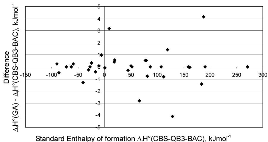
Figure 5. Differences between standard enthalpies of formation for alkenes from group additivity and from the CBS-QB3-BAC method (298 K, kJ mol -1 ).
