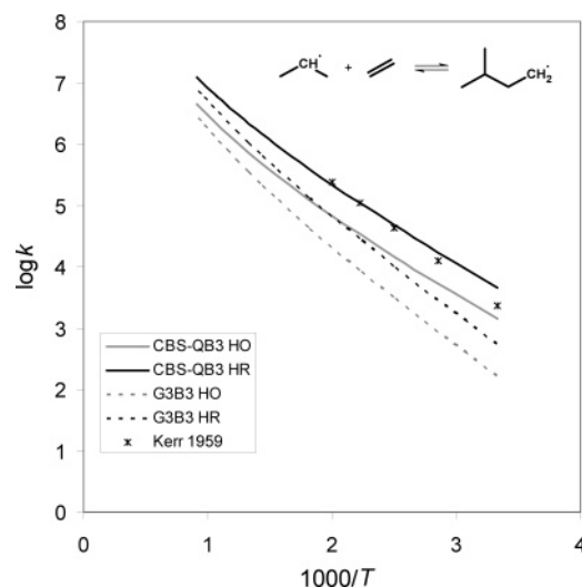
Figure 9. Arrhenius plot for the reaction \text{iso-C}_3\text{H}_7\cdot + \text{C}_2\text{H}_4 \rightarrow \text{C}_5\text{H}_{11}\cdot : CBS-QB3 and G3B3 rate coefficients in the HO and HR approach and comparison to experimental reference ( \text{m}^3 \text{kmol}^{-1} \text{s}^{-1} ).
