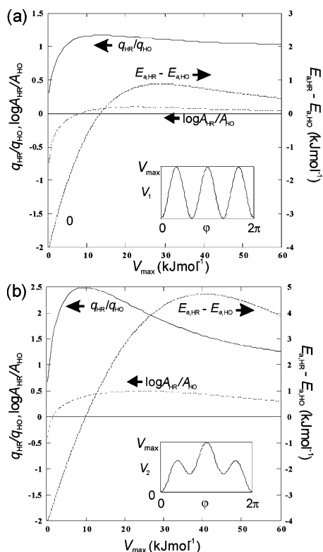
Figure 1. Influence on q , E_a , and \log A of the hindered internal rotor treatment of the internal rotation about the forming bond in the transition state for two model potential energy profiles for internal rotation ( I_{\text{red}} = 20 amu bohr 2 , T = 1000 K, \sigma = 3 and 1, respectively).
