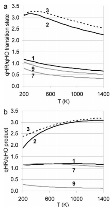
Figure 2. Ratios q_{\text{HR}}/q_{\text{HO}} vs T for (a) the transition state and (b) products of selected reactions.
