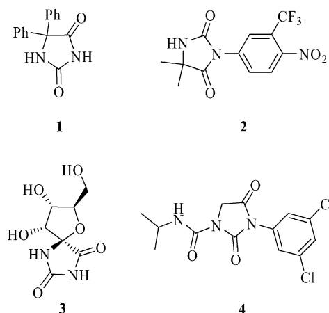
Figure 1. Phenytoin ( 1 ), nilutamide ( 2 ), hydantocidin ( 3 ) and iprodion ( 4 ).
