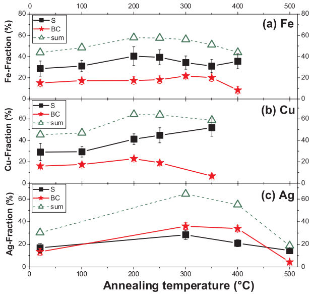
FIG. 2 (color online). Fraction of the implanted Fe (a), Cu (b), and Ag atoms (c) on the S site (■) and the BC site (★) in Ge, together with the total fraction ( \Delta = \blacksquare + \star ) on high-symmetry sites, as a function of annealing temperature.
