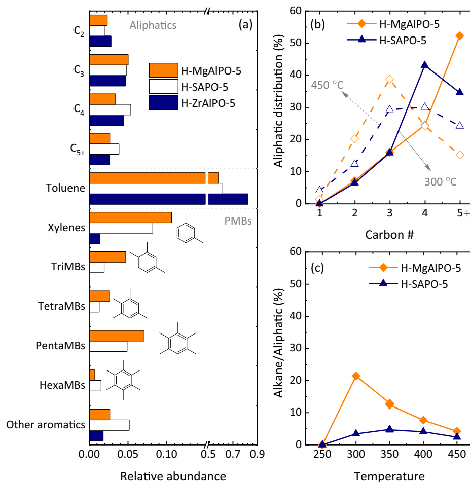
Fig. 5. (a) Reaction product distribution obtained at 400 °C with the H-MeAlPO-5 catalysts and effect of temperature on the (b) aliphatic distribution and (c) alkane-to-aliphatics ratio. GHSV = 34 (H-MgAlPO-5), 26 (H-SAPO-5) and 15 cm 3 g -1 s -1 (H-ZrAlPO-5). P_{\text{Benzene}} = 80 mbar, P_{\text{DME}} = 20 mbar.
