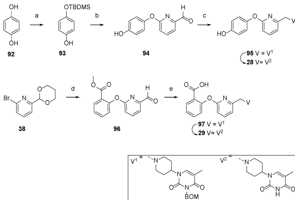
Scheme 3. Synthesis of derivatives of analogue 3 (analogue 28 and 29 ).
