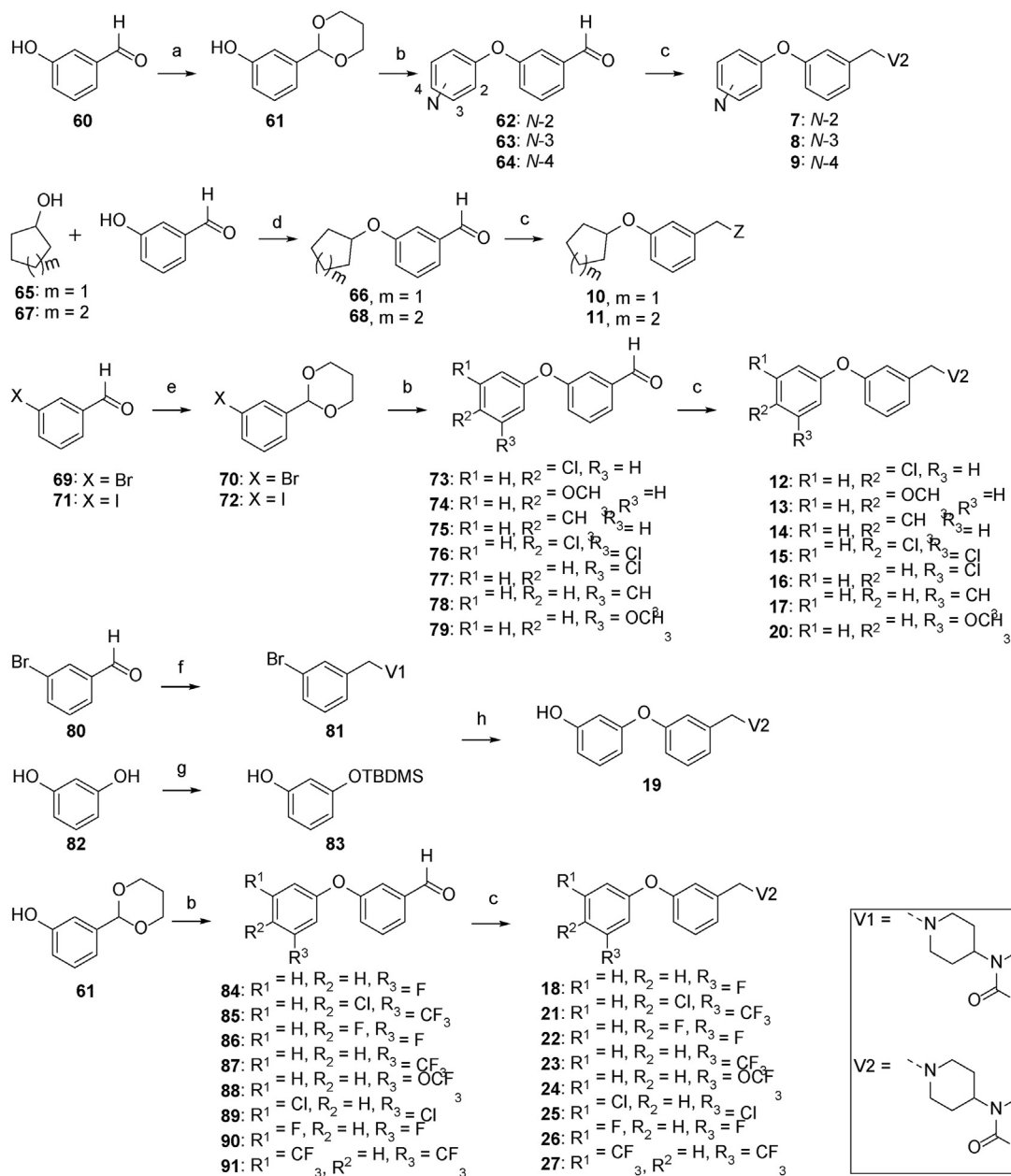
Scheme 2. Synthesis of D-ring modified derivatives (Series 2).
