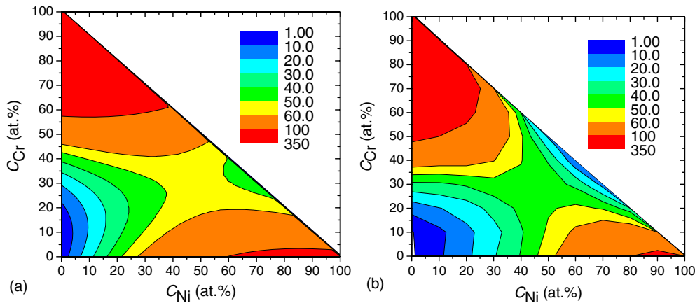
Figure 3. The stable SFE ( \text{mJ m}^{-2} ) as function of composition obtained from thermodynamic calculations [25] (a) and the potential (b).
