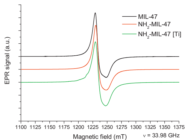
Fig. 10. Q-band (33.98 GHz) EPR spectrum of NH 2 -MIL-47 [Ti] compared with the spectra of non-functionalized NH 2 -MIL-47 and of MIL-47 at RT. (For interpretation of the references to color in the artwork, the reader is referred to the web version of the article.)
