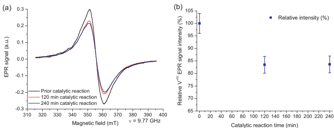
Fig. 9. (a) X-band EPR spectra at RT of the NH 2 -MIL-47 [Ti] samples before and after catalysis; (b) Relative V IV EPR signal intensity with respect to the signal of NH 2 -MIL-47 [Ti] prior to catalysis. The error (1 \sigma ) is estimated at 4% (see text). (For interpretation of the references to color in the artwork, the reader is referred to the web version of the article.)
