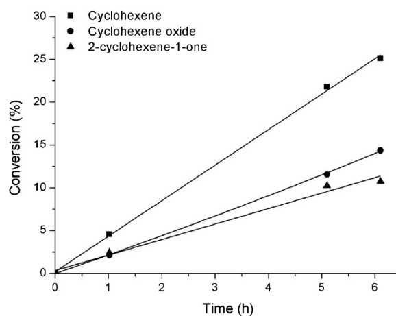
Fig. 7. Cyclohexene conversion (■) and the yield of cyclohexene oxide (●) and 2-cyclohexene-1-one (▲) for TiO(acac) 2 using acetonitrile as solvent and oxygen as oxidant in combination with the co-oxidant cyclohexanecarboxaldehyde at a temperature of 40 °C. The same Ti loading was applied as for the NH 2 -MIL-47 [Ti] (0.22 mmol Ti).
