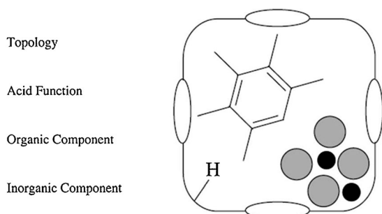
Figure 8. View of a single cage in a supramolecule zeolite catalyst for MTO conversion, with indication of its four key features as proposed by Haw et al. [96] (Reprinted with permission from ref. [96]. Copyright 2005 Springer.)
