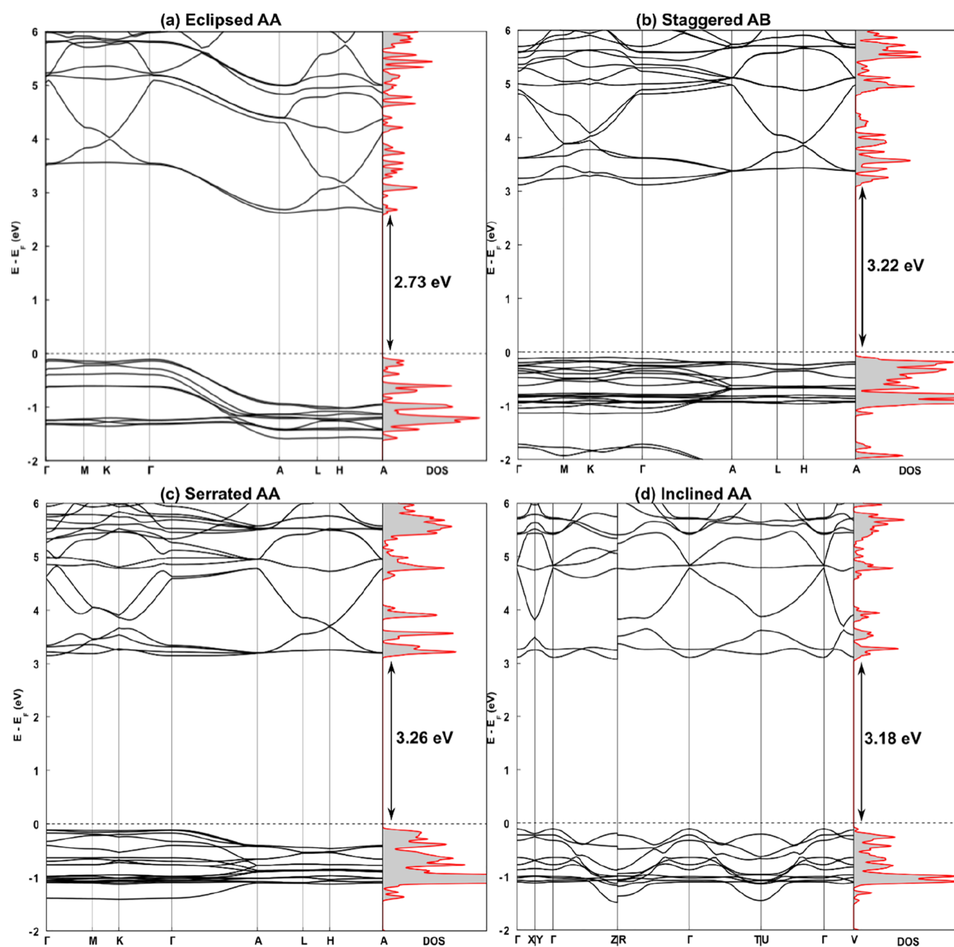
Figure 7. Band structure and density of states of (a) eclipsed AA-, (b) staggered AB-, (c) serrated AA-, and (d) inclined AA-stacking for CTF-1 using the HSE06 functional. The Fermi level is shifted to zero and specified by the gray dashed line.
