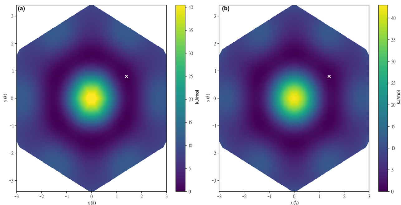
Figure 3. Contour plots visualizing the PES as a function of the layer offset vector for (a) inclined AA-stacking (at a fixed interlayer distance of 3.38 Å) and (b) serrated AA-stacking (at a fixed interlayer distance of 3.36 Å) in CTF-1 using PBE-D3(BJ). The white cross shows the most stable configuration. The unit cell consists of one layer and two layers for inclined and serrated stacking, respectively. The energy of the most stable configuration was set to zero for each stacking configuration separately.
