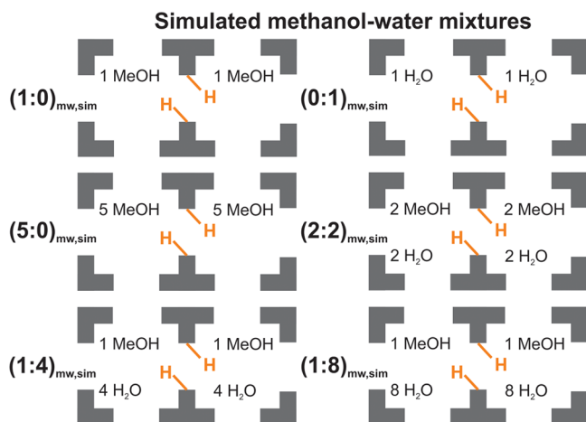
Scheme 2. Simulated Loadings of Methanol–Water Mixtures in H-SAPO-34 with Indication of the Acid Sites a
