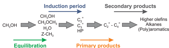
Scheme 1. Schematic of the Stages during Methanol Conversion over a Solid Acid Zeolite Based Catalyst a
