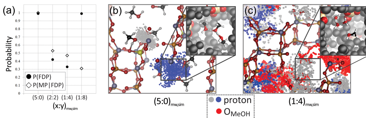
Figure 1. (a) Probability for framework deprotonation (FDP) and probability of methanol protonation when the framework is deprotonated (MPIFDP) during 50 ps MD simulations of different methanol–water mixtures adsorbed in H-SAPO-34 at 330 °C and around ambient pressure. (b, c) H-SAPO-34 loaded with a (5:0) mw,sim and (1:4) mw,sim methanol–water mixture. The gray, blue, and red dots represent the positions of the two acid protons and methanol oxygen atoms, respectively. The insets show snapshots of the MD run with highlighted acid sites. (x:y) mw,sim stands for a simulation with x MeOH and y H 2 O molecules per BAS.
