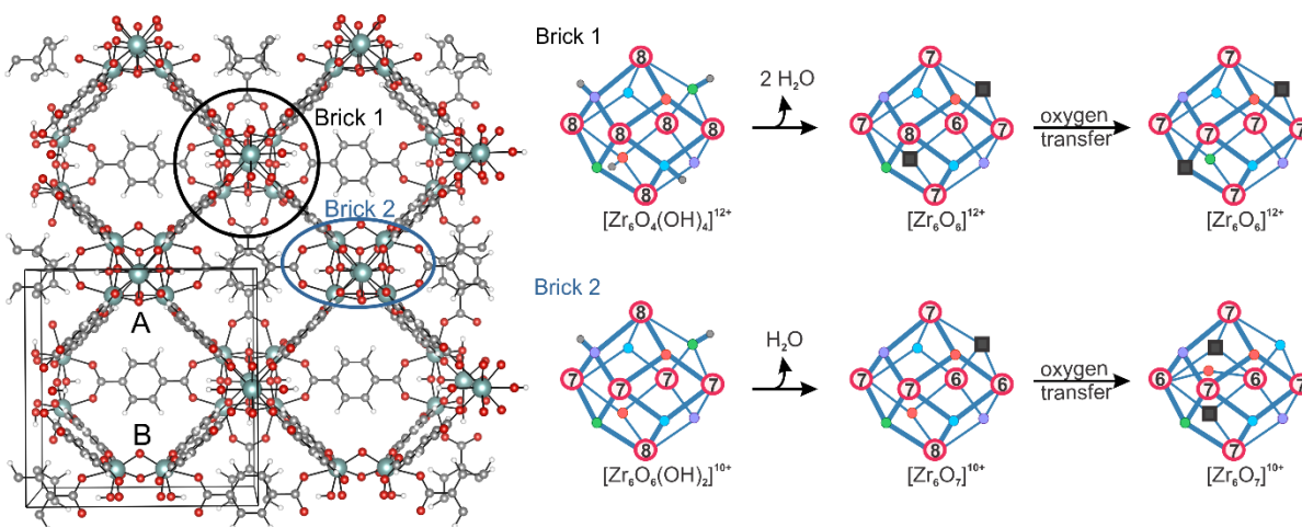
Figure 1: Periodic model of UiO-66 with indicated unit cell and encircled two types of bricks. Zr-brick 1 with formula [Zr_6O_4(OH)_4]^{12+} is intact without missing linker, while brick 2 [Zr_6O_6(OH)_2]^{10+} has in total two terephthalate linkers missing, one at site A and one at the opposite site B. On the right, the dehydration processes of brick 1 and brick 2 are shown. Coordination number of different Zr atoms in the brick are encircled in red. Oxygen vacancies are displayed as grey squares.
