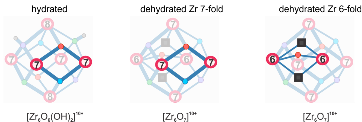
Figure 4: Representation of active sites for catalysis in brick 2 on the hydrated and dehydrated UiO-66. Oxygens are represented by medium circles. Their color can differ but has no real physical significance and originates from ref. [5b]
