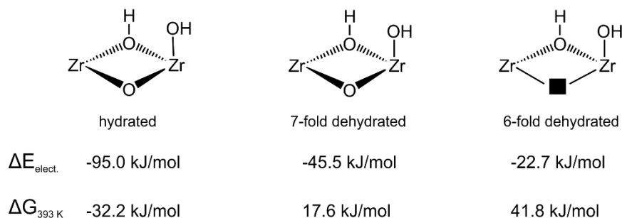
Figure 6: Influence of water coordination on the three active sites (hydrated Zr(7)-O-Zr(7), dehydrated 7-fold Zr(7)-O-Zr(7) and dehydrated Zr(6)-O-Zr(6) UiO-66).
