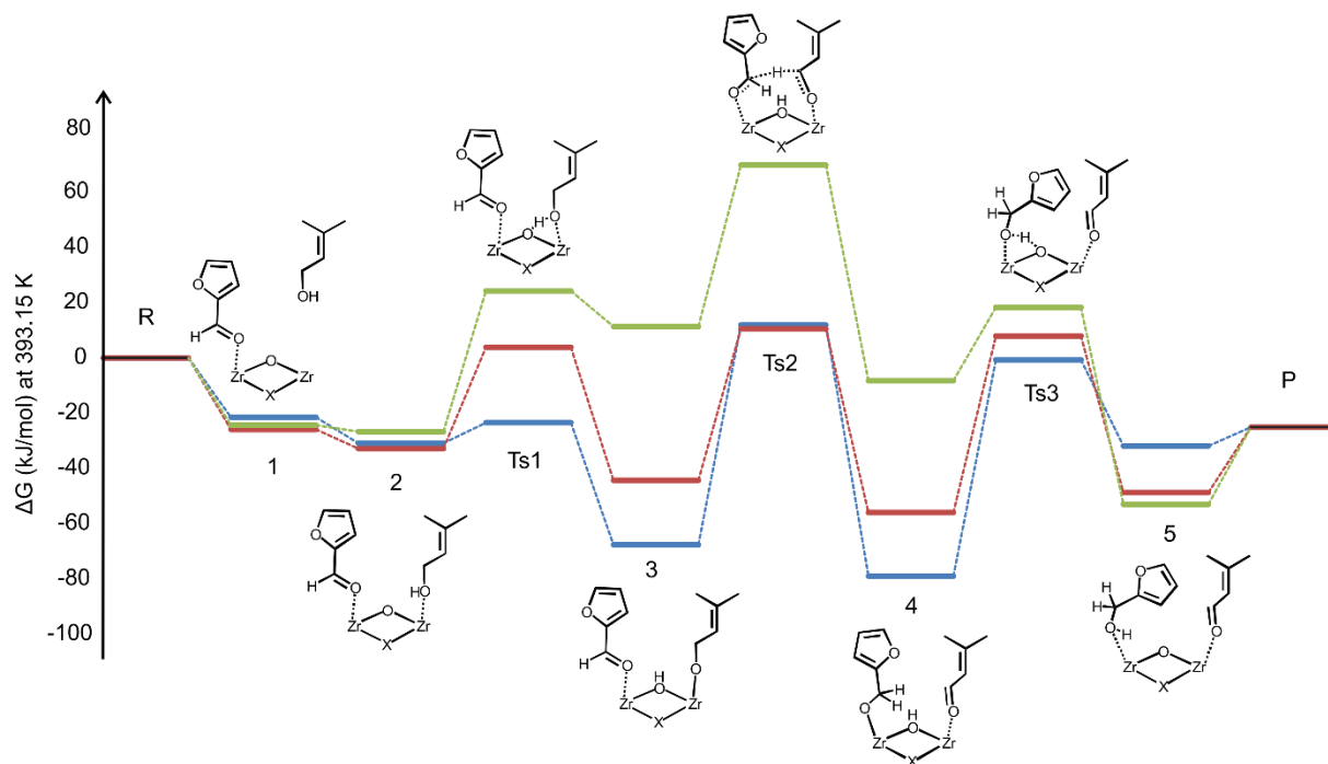
Figure 5: Free energy profile of the Oppenauer oxidation of prenil with furfural (periodic with PBE-D3) given at 393.15 K. Hydrated brick is indicated by a blue line, while dehydrated 7- and 6-fold coordinated Zr by a red and green line, respectively. X corresponds to: X=O in the hydrated and dehydrated 7-fold material, and X=vacancy for the cluster with 6-fold Zr coordination. R corresponds to the reactants in gas phase and the catalyst, P corresponds to the final products in gas phase and the catalyst.
