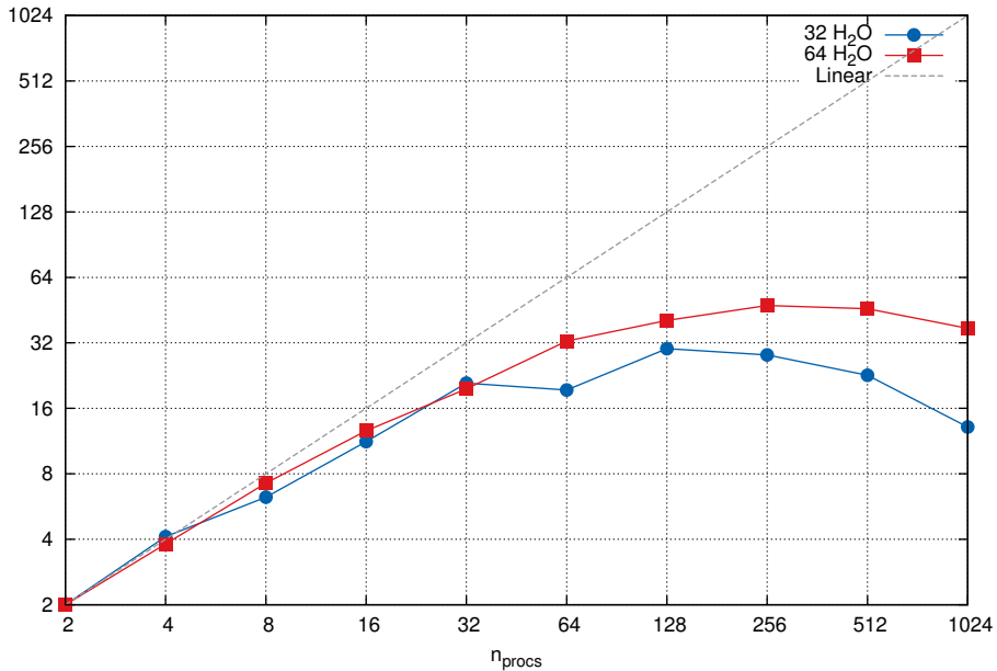
Scaling test on tier1 - GAPW
