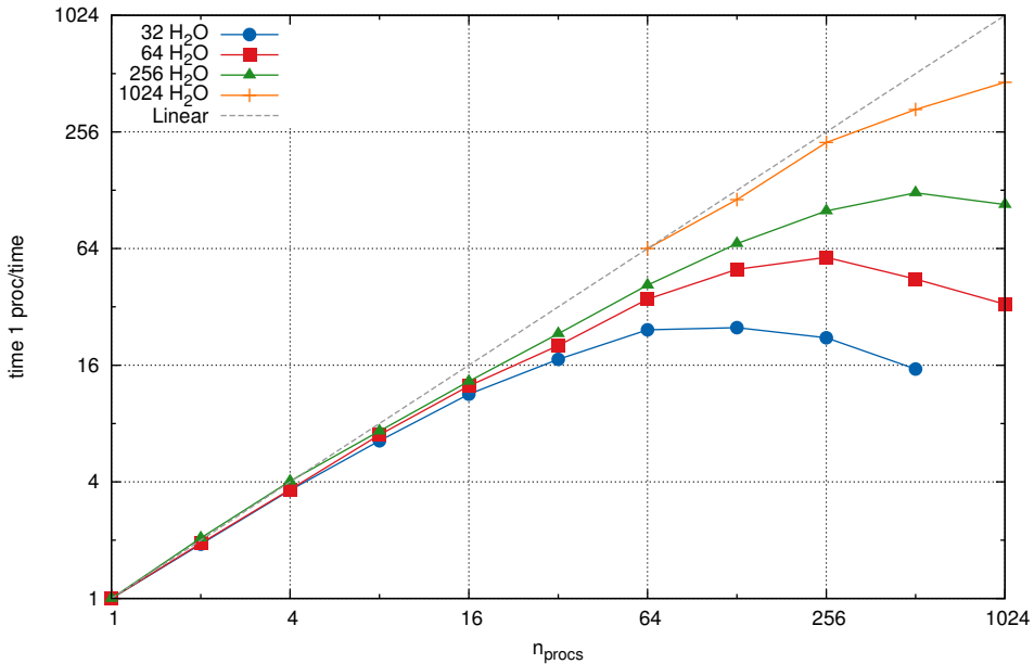
Scaling test on tier1 - GPW scheme
