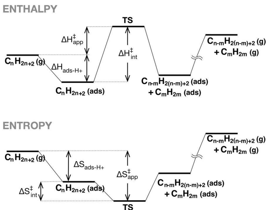
Figure 2. Schematic enthalpy and entropy landscapes illustrating the various steps in monomolecular reactions of alkanes in a Brønsted acid zeolite: the alkane adsorbs onto an active site, is converted into an alkene and a smaller alkane (cracking, m < n ) or H_2 (dehydrogenation, m = n ), and the cracking or dehydrogenation products desorb from the active site. Apparent activation parameters ( \Delta H_{app}^\ddagger and \Delta S_{app}^\ddagger ) extracted directly from experimental measurements are determined by both the adsorption enthalpy ( \Delta H_{ads-H^+} ) and adsorption entropy ( \Delta S_{ads-H^+} ) of the reactants at the Brønsted acid sites and the intrinsic activation parameters ( \Delta H_{int}^\ddagger and \Delta S_{int}^\ddagger ) associated with the chemical transformation at the active site.
